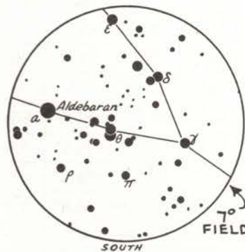
THE HYADES - ERECT VIEW AS SEEN WITH 7x BINOCULAR (7° FIELD)
